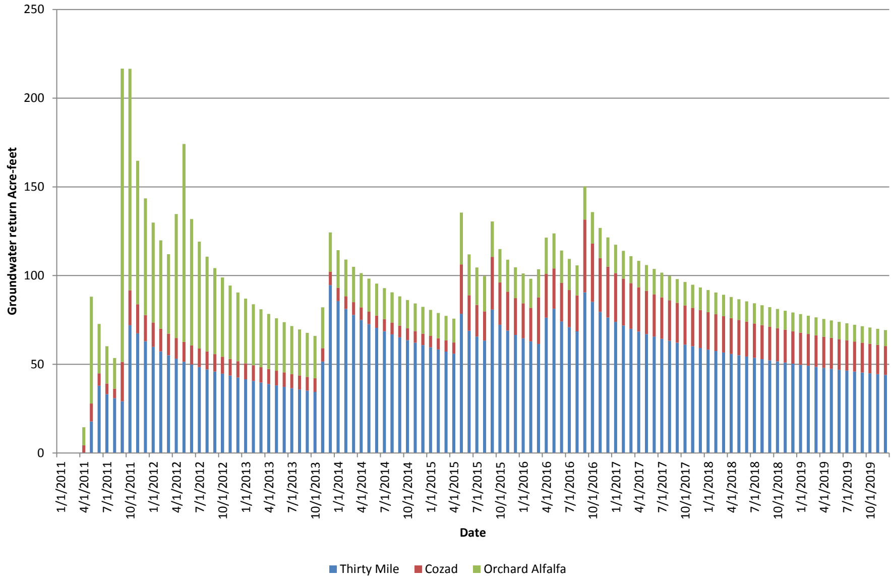
Figure 2. Base flow return from Excess River flow diversion and recharge by Canal
