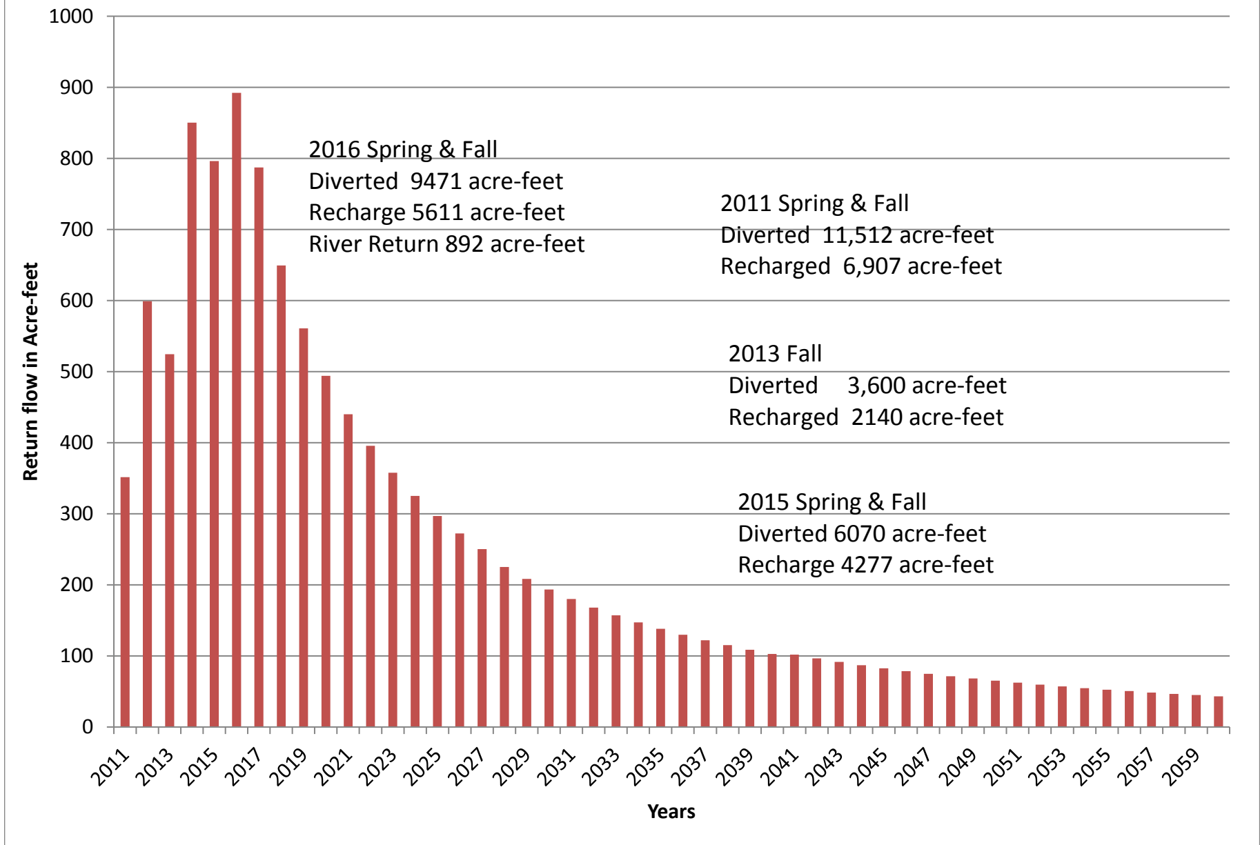
Figure 3. Thirty Mile Canal Excess Flow Return to Platte River as baseflow
